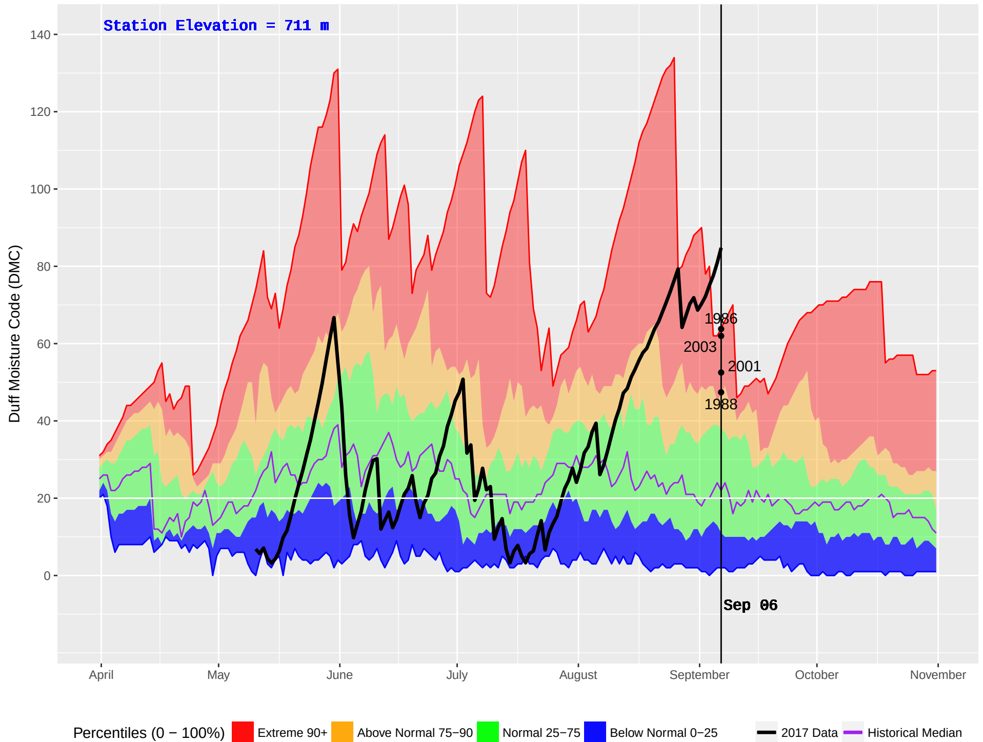
TOAD RIVER (126) : Historical (1981–2016) and Current (2017) Noon Duff Moisture Code (DMC)
