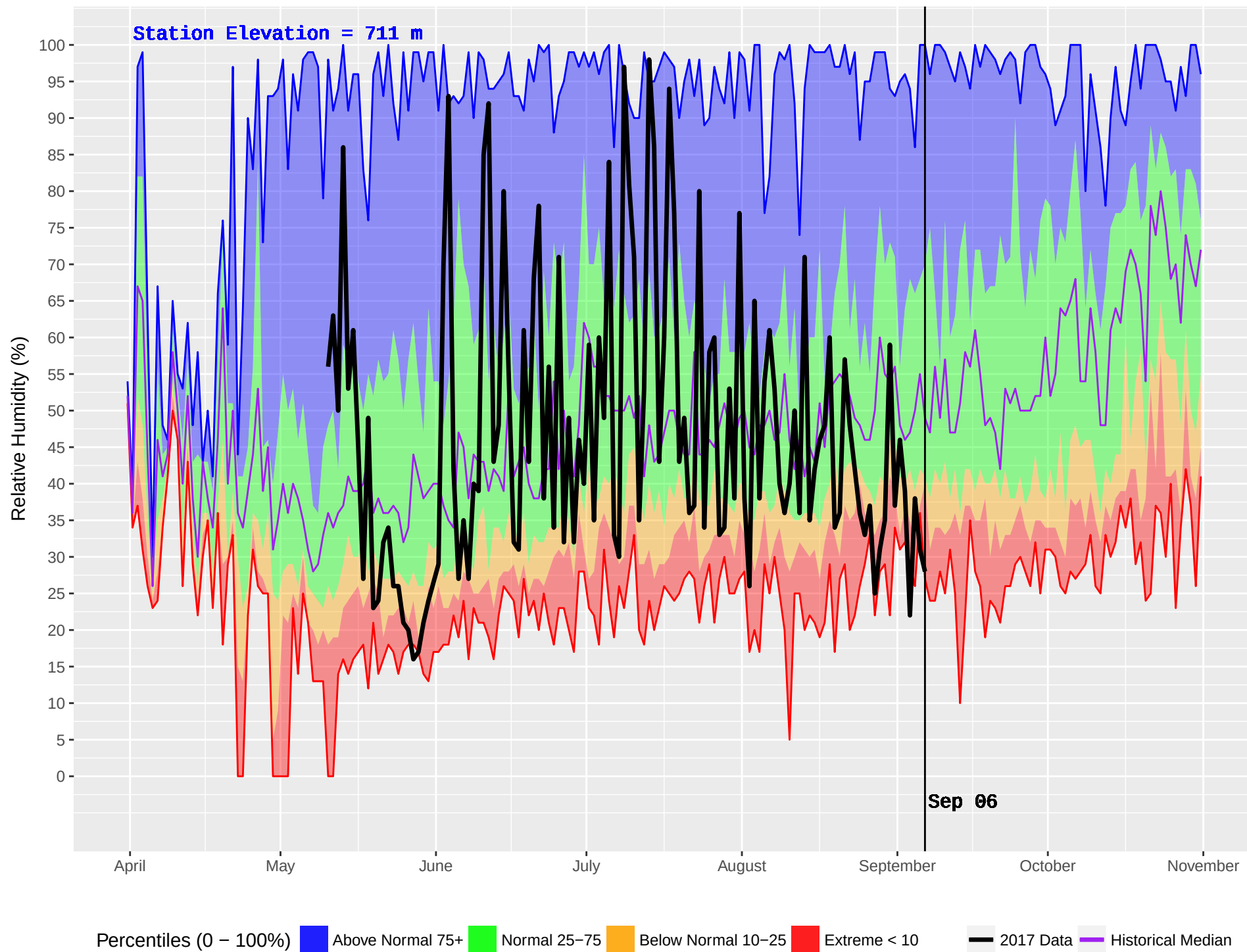
TOAD RIVER (126) : Historical (1981–2016) and Current (2017) Noon Relative Humidity
