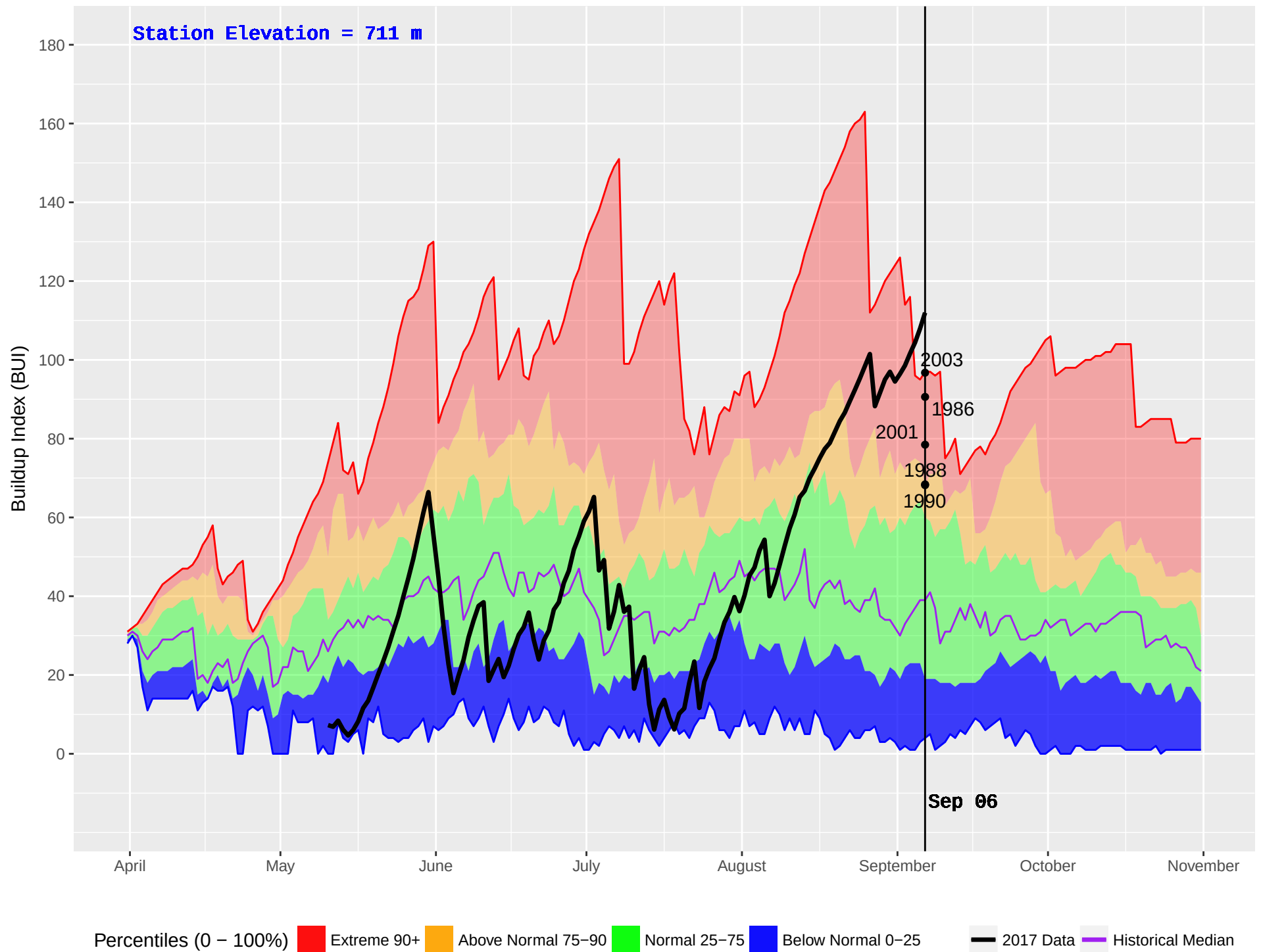
TOAD RIVER (126) : Historical (1981–2016) and Current (2017) Noon Buildup Index (BUI)
