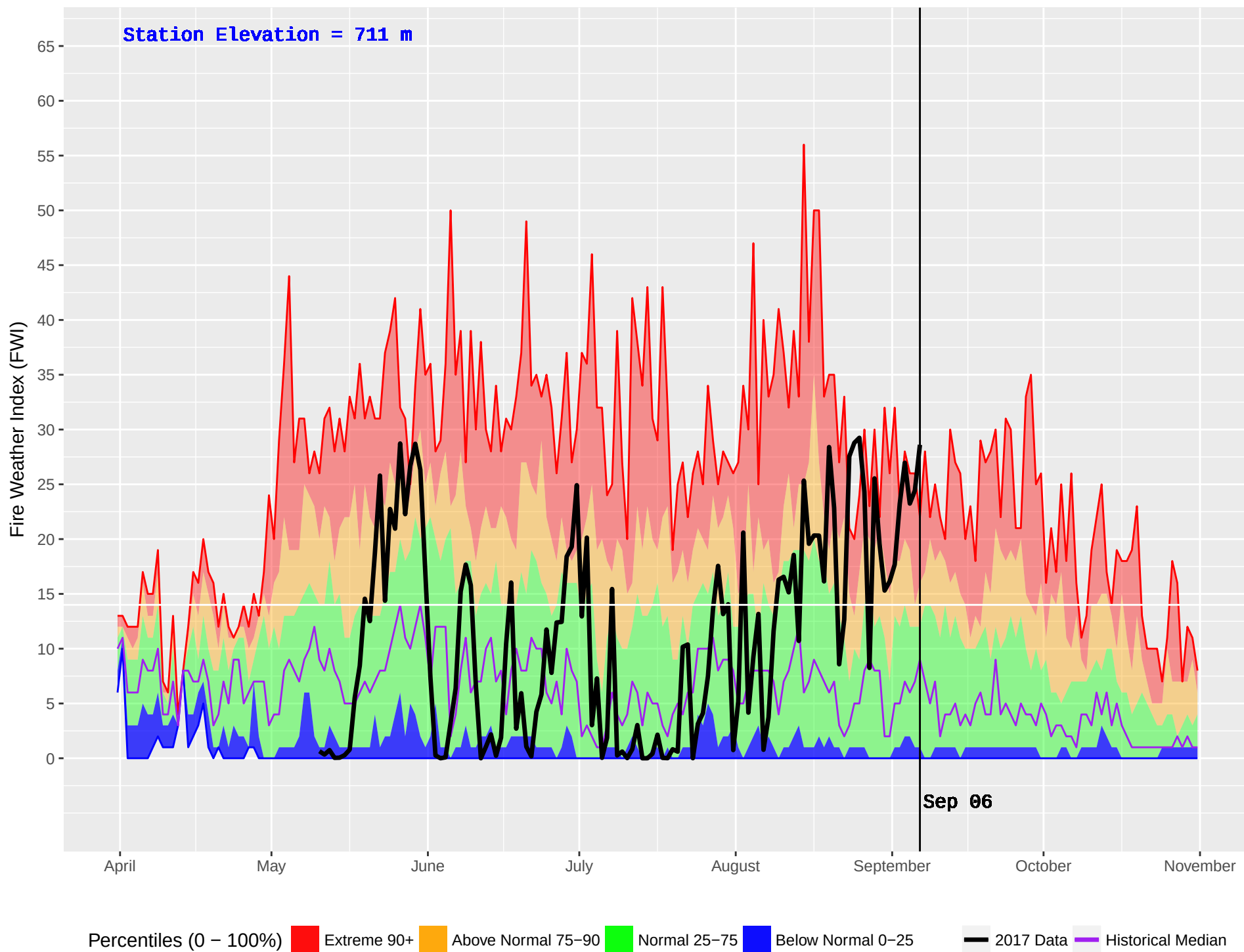
TOAD RIVER (126) : Historical (1981–2016) and Current (2017) Noon Fire Weather Index (FWI)
